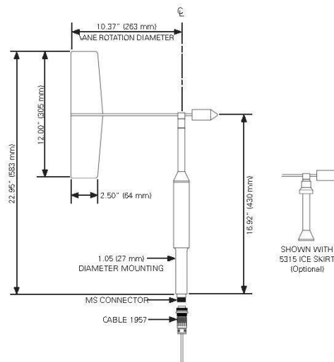
020D Wind Direction Sensor
